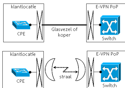
Figuur 2: Standard Access
